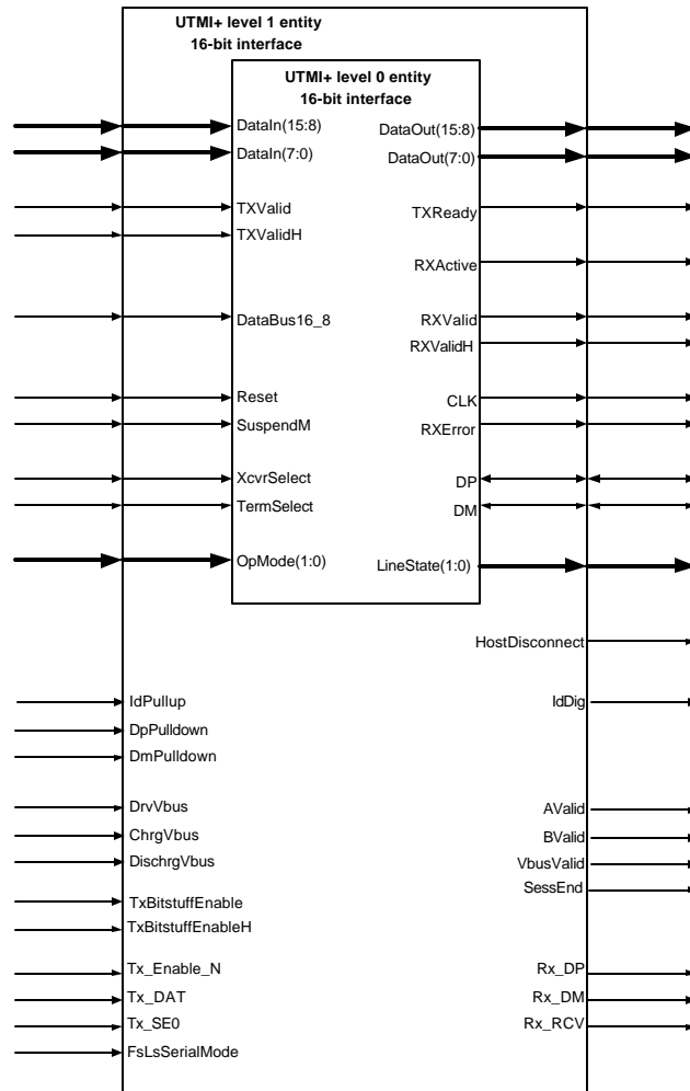
Figure 3 : UTMI+ level 1 entity diagram
