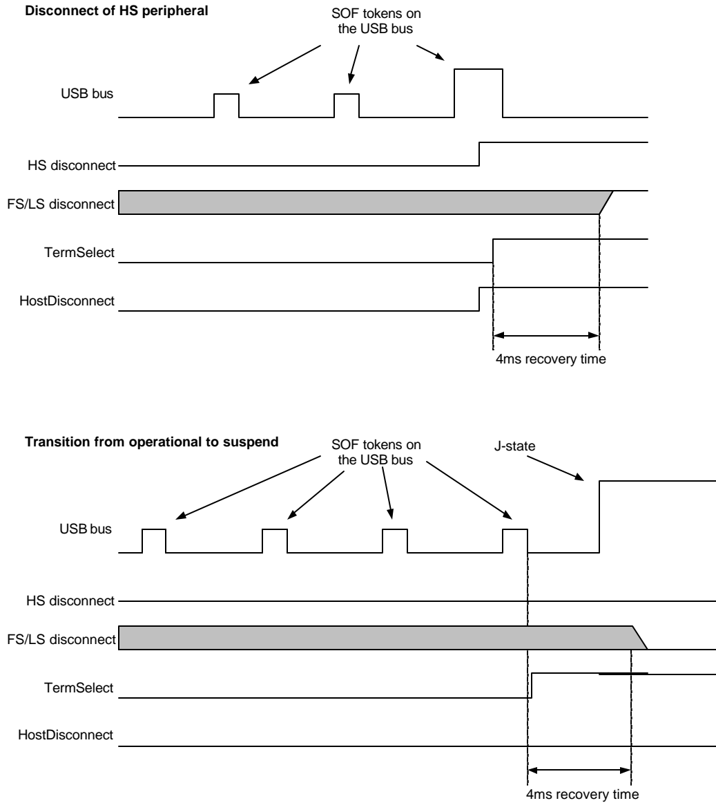
Figure 4 : HostDisconnect behaviour (signals are not on scale)
