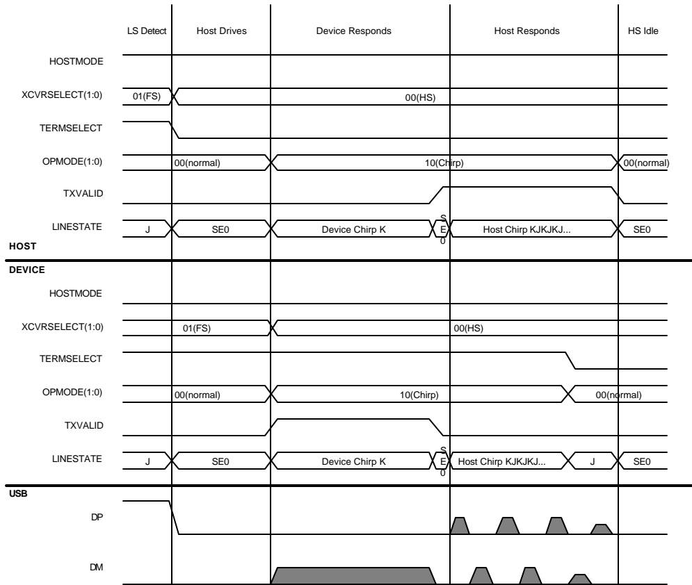
Figure 8 : Reset sequence for a HS peripheral connected to a HS Host Controller
