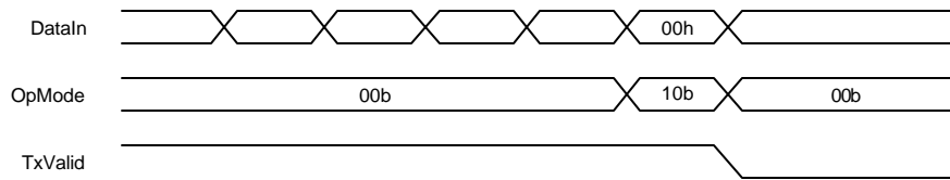
Figure 10 : Transmit error reporting for downstream facing ports
