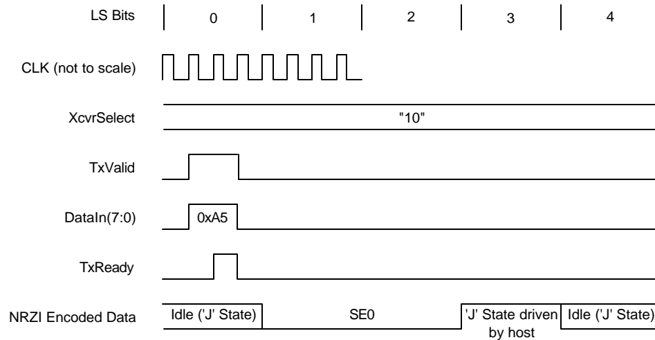
Figure 7 : LS keep-alive generation
