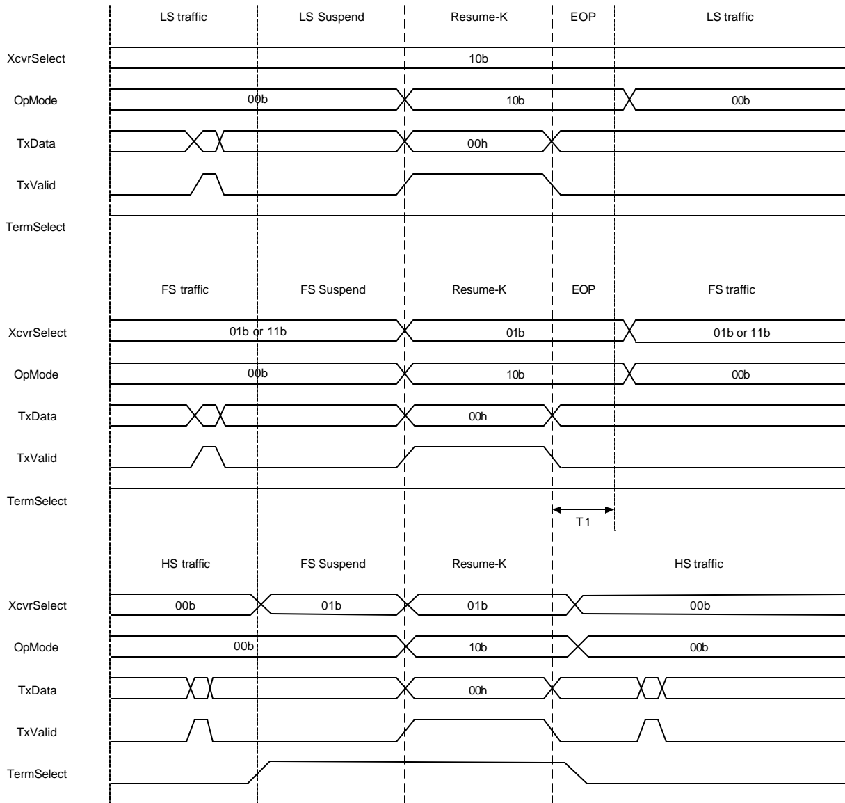
Figure 9 : Resume signaling on downstream facing ports
